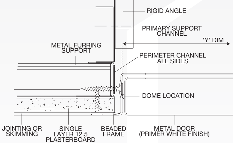
Fig.4 scale 1:2 section on B
