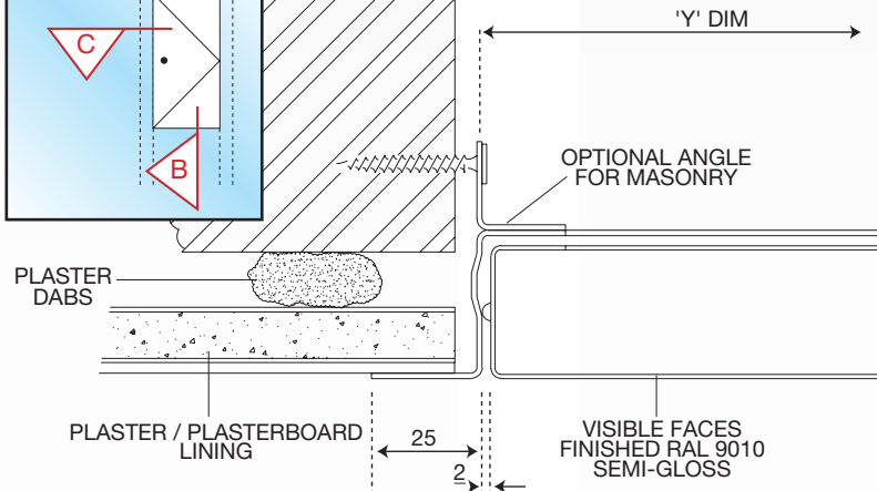
Fig.5 scale 1:2 section on C
